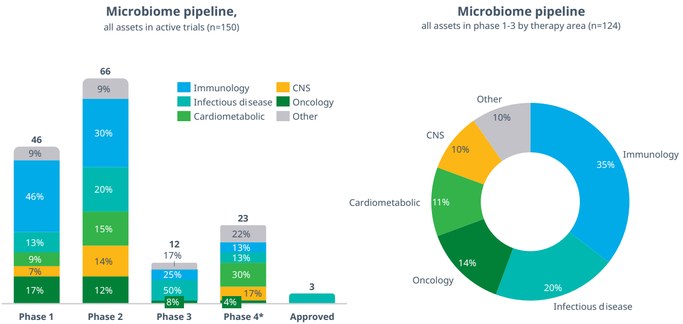
Figure 1: Microbiome Pipeline
